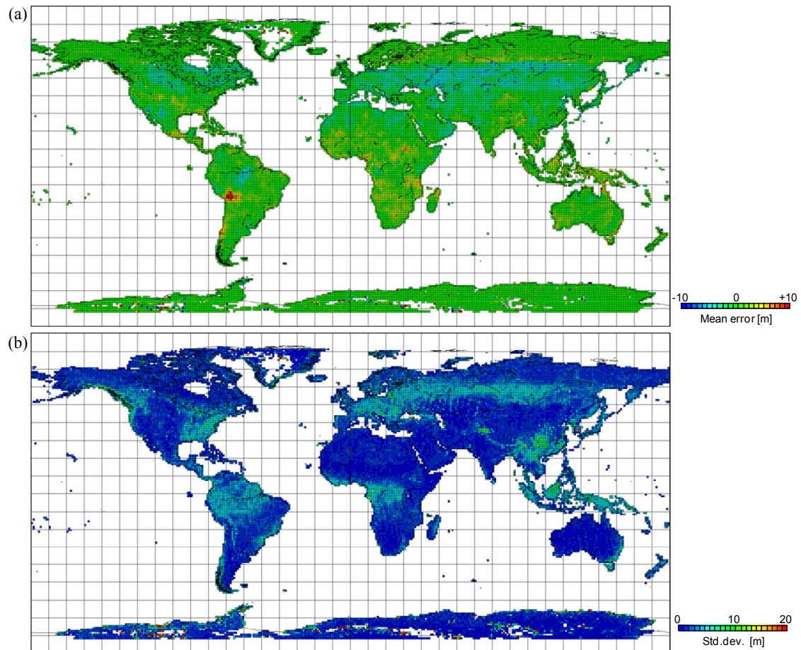
Figure 3. Distribution of mean errors (a) and error standard deviations (b) from ICESat data points for DSM-tiles.
