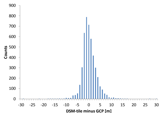
Figure 5. Histogram of the height differences from 4,628 GCPs.
