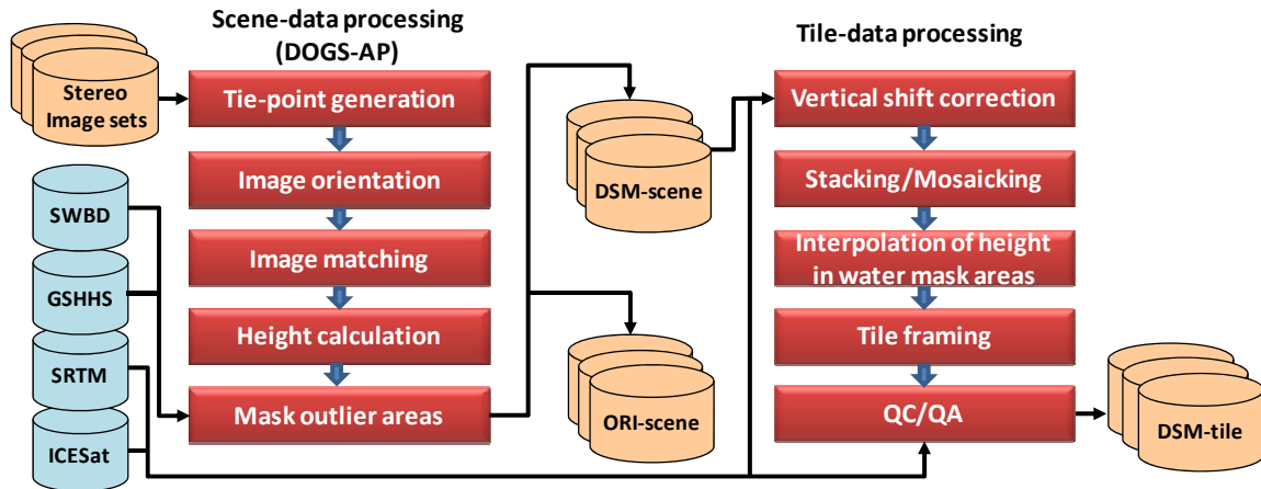
Figure 1. Processing flow of the ‘AW3D’ global DSM datasets.
