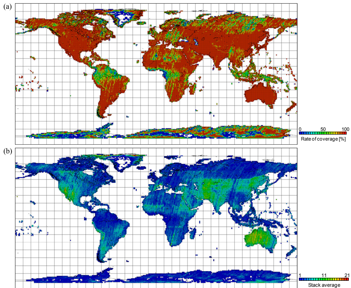
Figure 2. Distribution of coverage rates R (a) and stack averages S (b) for DSM-tiles.
