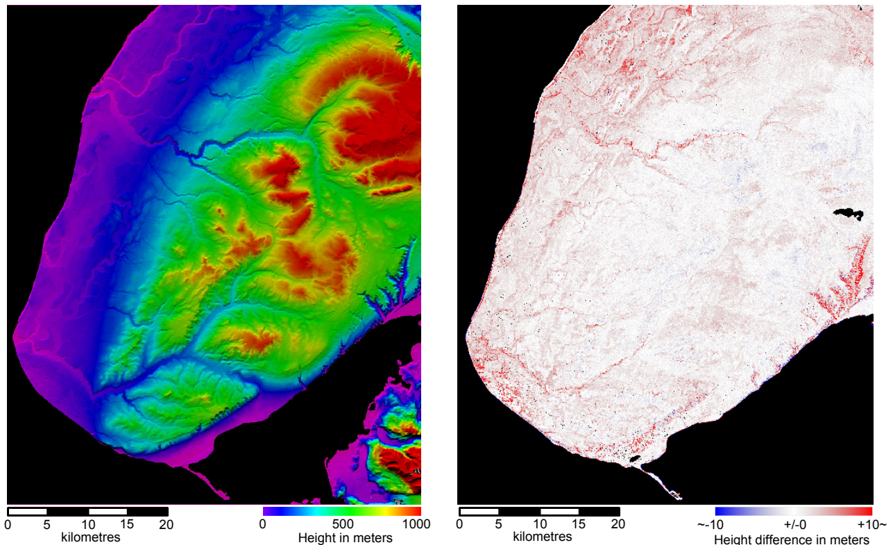
Figure 6. Painted relief image of the DSM-tile data on the validation area, which has the height range of approx. 0~900 m, selected from the reference LiDAR/DEM (left) and the height difference image between DSM-tile data and the reference LiDAR/DEM data (DSM-tile minus LiDAR/DEM) (right). The black areas in the painted relief image represent the mask of the sea, while ones in the difference image represent masks which were not used in the validation.
