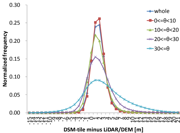
Figure 7. Histogram of height differences for different ranges of slope angles as well as for whole data. The depicted difference-range corresponds to \pm 3\sigma from the \mu for the distribution in the slope range of 30 \leq \theta .
